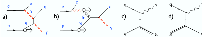
Fig. 1. Examples of LO graphs for prompt photon production in \gamma p (a,b) and hadron-hadron interactions (c,d).
